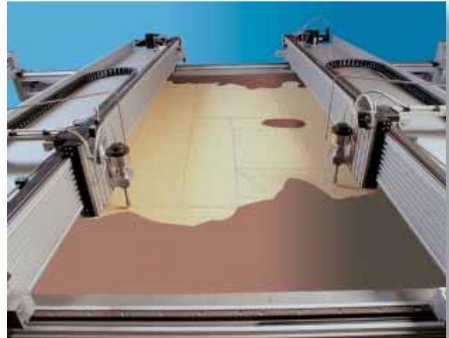
Simultaneous cutting of one leather hide with two cutting heads.
